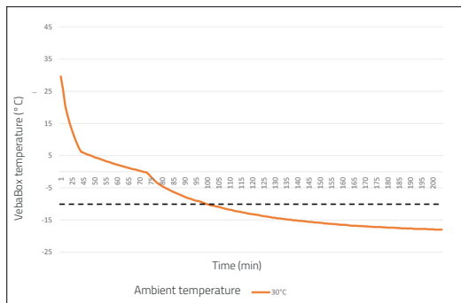
Cooling performance at ambient temperature Model F Freeze
