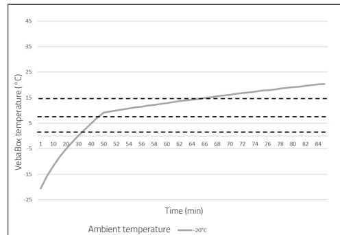
Heating performance at ambient temperature Model F Freeze
